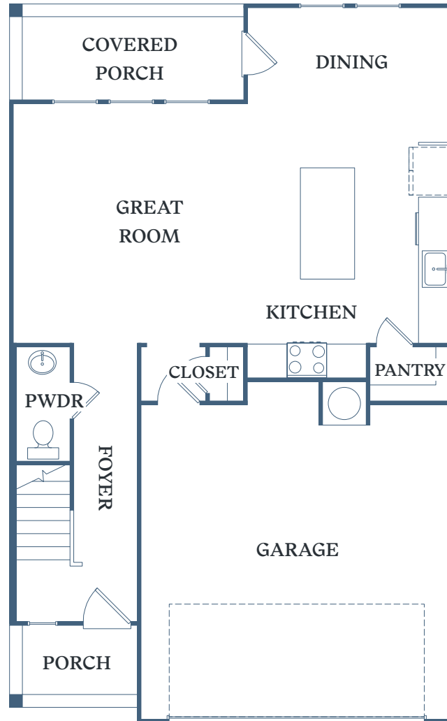
1 ST FLOOR – 646 SF
